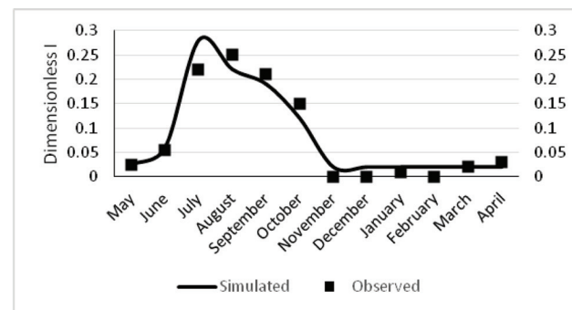
Figure 2.1. Simulated values vs. observed values for the Leptospirosis infected population in Nakhon Ratchasima-Year 2000.
