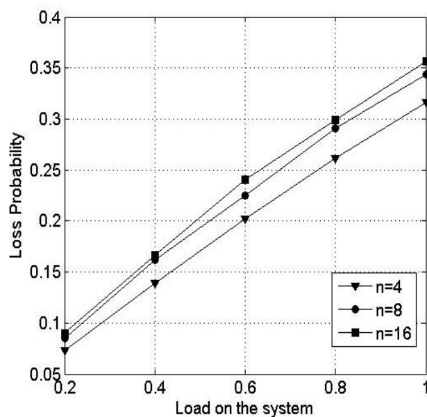
Figure 5. The burst loss probability vs. load with buffering of zero burst, and Burst Length of four while varying the number of nodes.
