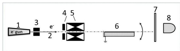
Figure 1. Experimental setup. 1 – electron gun, 2 – beam of electrons, 3 – collimator Ø 2 mm, 4 – solenoid magnetic lens, 5 – magnetic corrector, 6 – target in the goniometer, 7 – screen, 8 – cam
