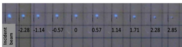
Figure 5. Displacement of the beam trace on the screen under tilting of the plate for the cross direction of the beam with respect to surface structure.
