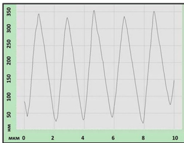
Figure 2. Profile of aluminum diffraction grating.
