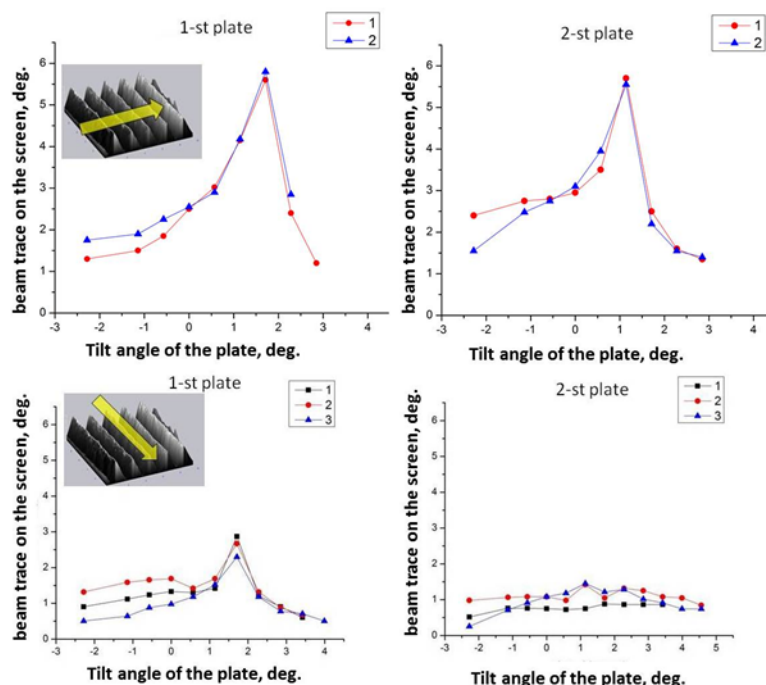
Figure 4. Displacement of the beam trace on the screen under tilting of two identical plates (left and right columns) for different directions of the beam with respect to surface structure (rows). Curves 1,2 and 3 on each plot correspond to different sets of experiments.
