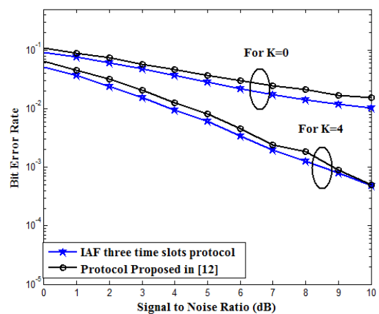
Figure 3. BER comparison of IAF protocol with protocol in 12 using variable SNR and different persistent K data values.
