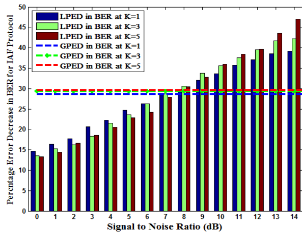
Figure 12. The GPED and LPED of IAF protocol compared to protocol in 15 , at persistent K values and variable SNR.
