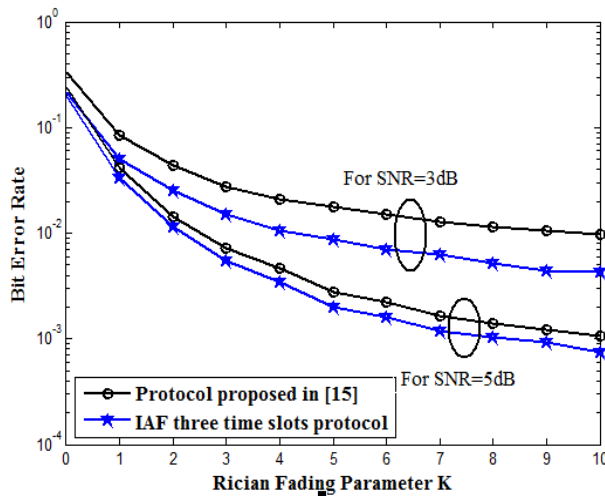
Figure 9. BER assessment of IAF protocol and protocol in 15 using variable K values and persistent SNR values.
