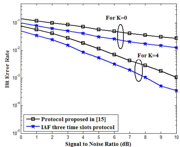
Figure 7. BER assessment of IAF protocol with protocol in 15 using variable SNR and persistent K values.
