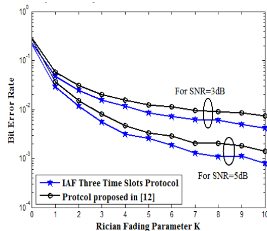
Figure 5. BER comparison of IAF protocol with previous protocol in 12 using variable K values and persistent SNR.
