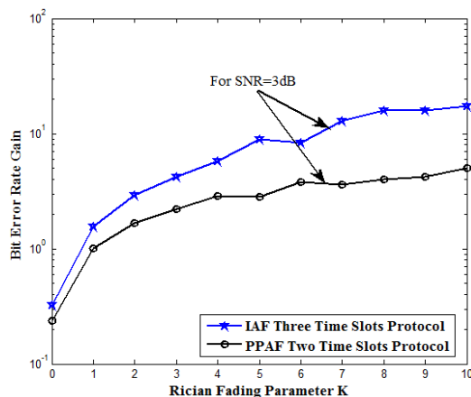
Figure 6. BER-Gain assessment of IAF protocol with protocol proposed in 12 using variable K data values and persistent SNR.
