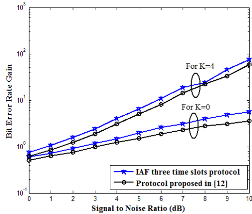
Figure 4. BER-Gain assessment of IAF protocol with protocol in 12 using variable SNR and persistent K data values.
