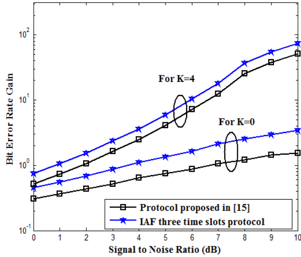
Figure 8. BER-Gain assessment of IAF protocol with protocol in 15 using variable SNR and persistent K values.
