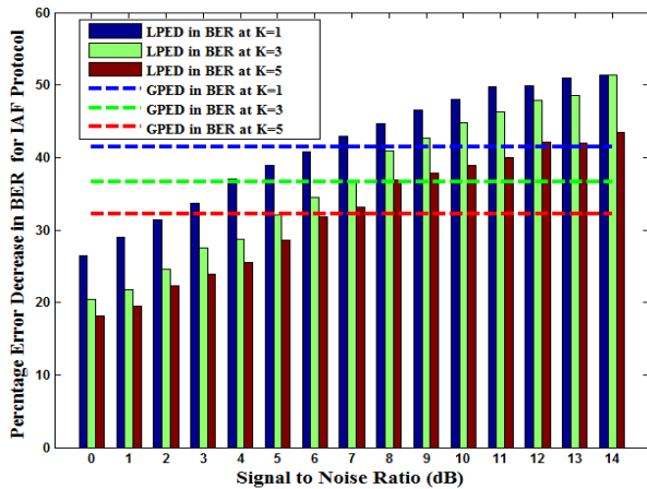
Figure 11. The LPED and GPED of IAF protocol compared to protocol in 12 , using persistent K values and variable SNR.
