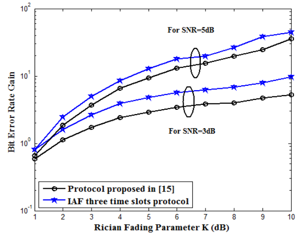
Figure 10. BER-Gain assessment of IAF protocol and protocol in 15 , using variable K values and persistent SNR.
