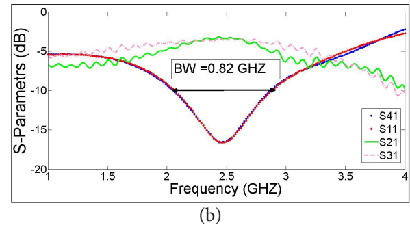
Figure 4. The measured S-parameters for (a) standard coupler (b) modified coupler.
