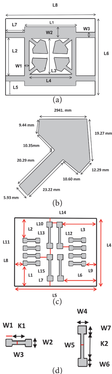
Figure 2. Geometry of the branch line coupler (a) conventional (b) modified (c) Geometry of the shape added into inner area of the 3dB coupler (d) The ground of the modified branch – line coupler.
