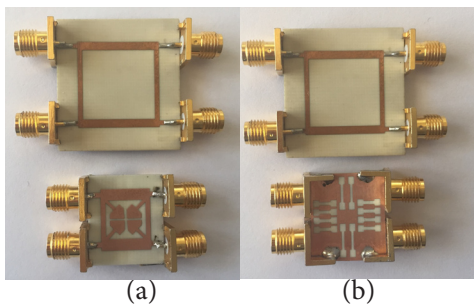
Figure 3. Branch line coupler (a) standard and modified top view (b) standard and modified bottom view.
