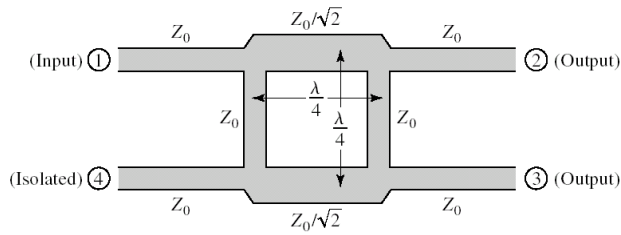
Figure 1. Geometry of a branch –line hybrid coupler.
