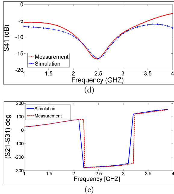
Figure 5. The simulation and measurement results for modified 3dB coupler.
