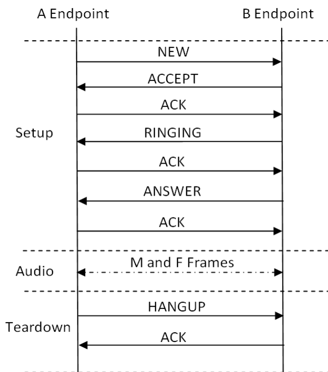
Figure 1. IAX-to-IAX communications 40 .
