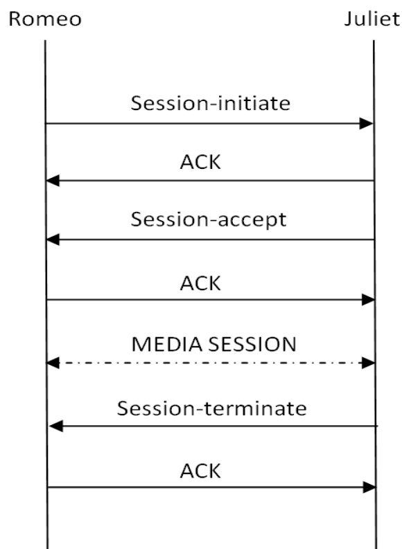
Figure 2. XMPP-to-XMPP communications 32 .
