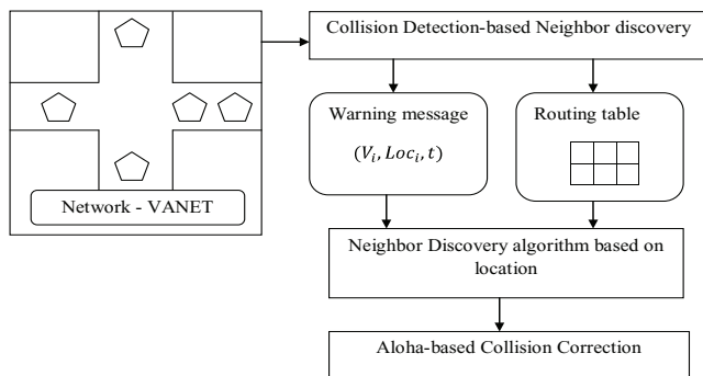
Figure 1. Block diagram of Neighbor Discovery based Collision Detection and Aloha-based collision correction.
