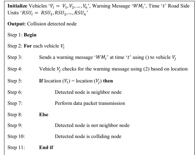
Figure 3. Neighbor discovery algorithm.
