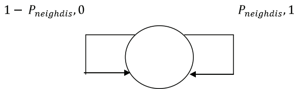
Figure 4. Aloha-based random model.
