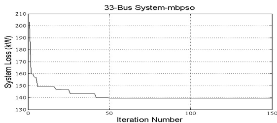
Figure 6. Convergence behaviour of BPSO algorithm.
