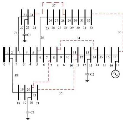
Figure 5. Test system.
