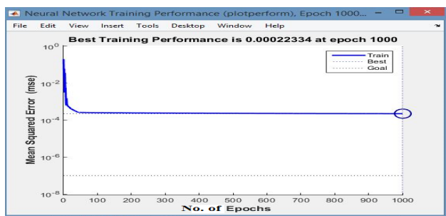
Figure 11. Training performance graph for logsig, trainrp.
