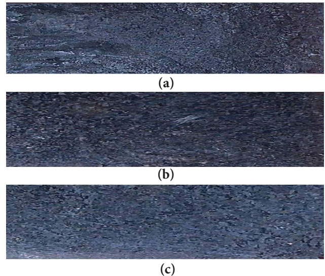
Figure 3. Investigating macrostructures of the obtained samples: a – sample No.1, ( \times 6 ); b – sample No.2, ( \times 6 ); c – sample No.3, ( \times 6 ).
