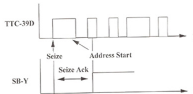
Figure 4. Handshake when TTC- 39D calls SB-Y.
