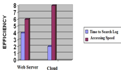
Figure 2. Performance measures.
