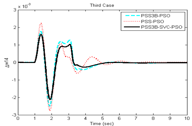
Figure 15. Inter-area mode ( W_1-W_4 ) of oscillation for case 3.
