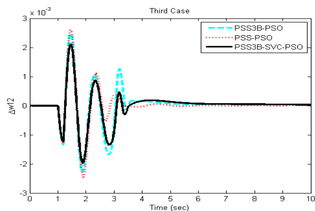
Figure 13. Local mode ( W_1-W_2 ) of oscillation for case 3.
