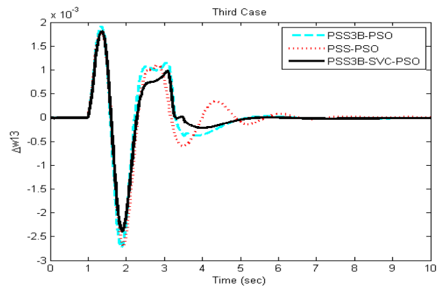
Figure 14. Inter-area mode ( W_1-W_3 ) of oscillation for case 3.
