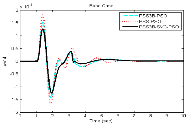
Figure 7. Inter-area mode ( W_1-W_4 ) of oscillation for case 1.
