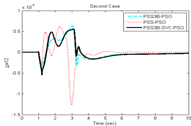
Figure 9. Local mode ( W_1-W_2 ) of oscillation for case 2.
