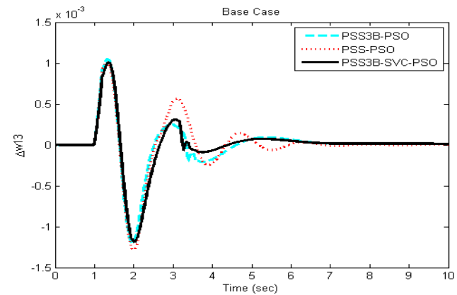
Figure 6. Inter-area mode ( W_1-W_3 ) of oscillation for case 1.
