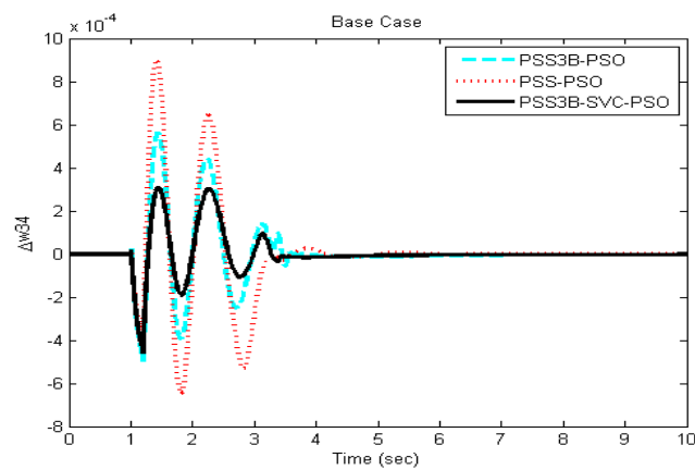
Figure 8. Local mode ( W_3-W_4 ) of oscillation for case 1.
