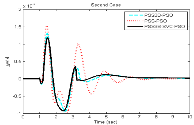
Figure 11. Inter-area mode ( W_1-W_4 ) of oscillation for case 2.
