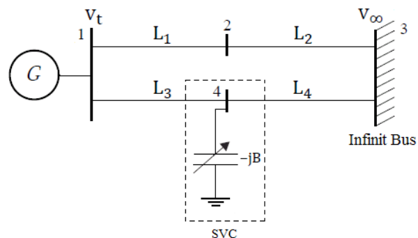
Figure 4. The structure of SVC.
