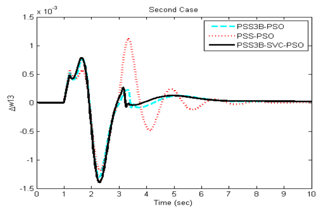
Figure 10. Inter-area mode ( W_1-W_3 ) of oscillation for case 2.
