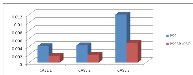
Figure 17. Value of performance index ISTSE for different case study.
