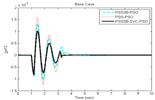
Figure 5. Local mode ( W_1-W_2 ) of oscillation for case 1.
