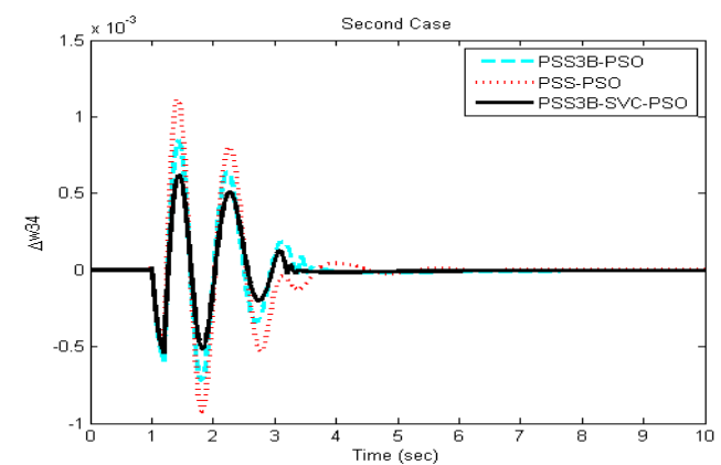
Figure 12. Local mode ( W_3-W_4 ) of oscillation for case 2.
