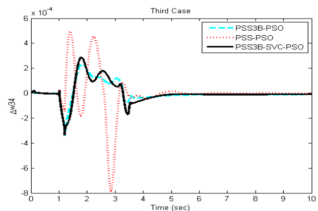
Figure 16. Local mode ( W_3-W_4 ) of oscillation for case 3.
