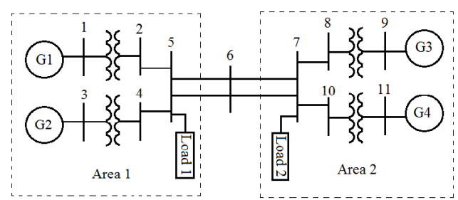
Figure 1. Multi-machine power system, IEEE.
