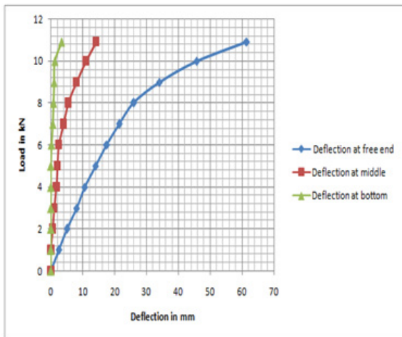
Figure 12. Load vs. Deflection of 30% Preloaded and Retrofitted with BFRP Hoop Directional Wrapped Elements.
