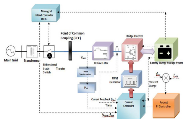
Figure 2. Configuration of Battery Energy Storage System (BESS).
