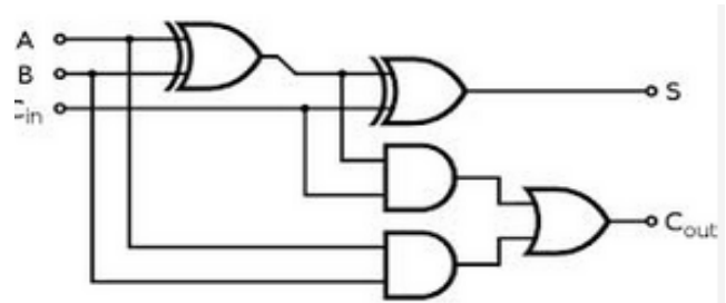
Figure 3. Full adder as sub module in the architecture.
