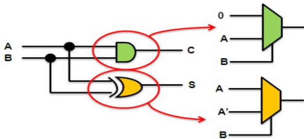
Figure 4. Half adder implementation using MUX.
