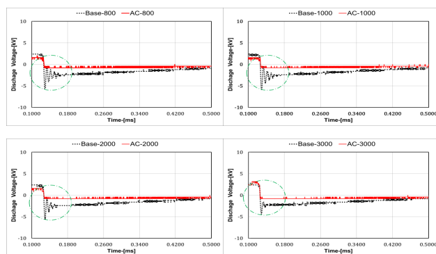
Figure 5. Discharge delay characteristics according to engine speed (rpm).
