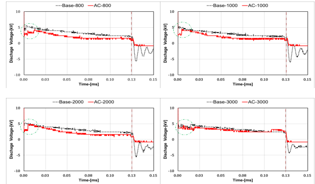
Figure 3. Discharge voltage characteristics according to engine speed (rpm).
