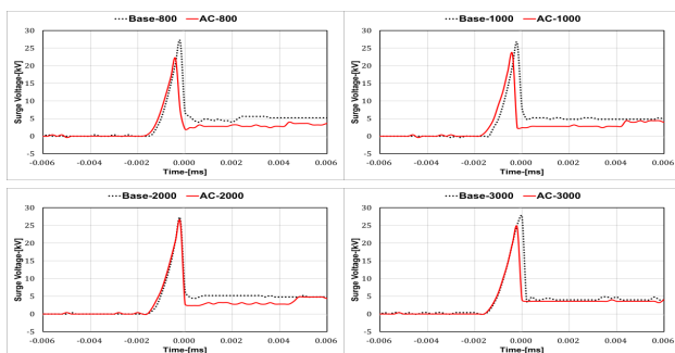
Figure 2. Surge voltage characteristics according to engine speed (rpm).
