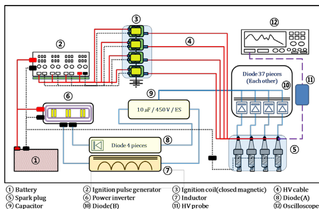
Figure 1. Schematic diagram of experimental device.
