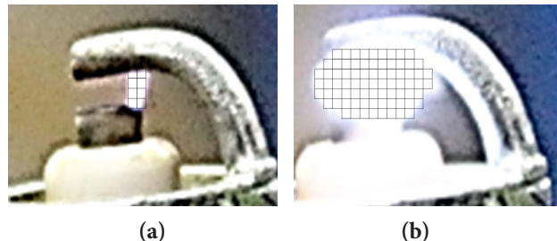
Figure 4. Comparison of ignition cross sections at 800rpm (a) Point ignition and (b) AC power ignition.
