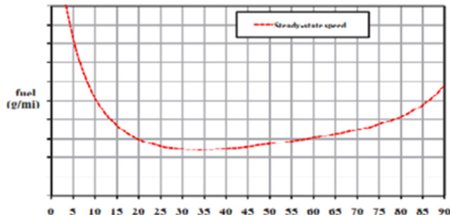
Figure 1. Fuel consumption versus average cruise speed generalized functional relationship.
