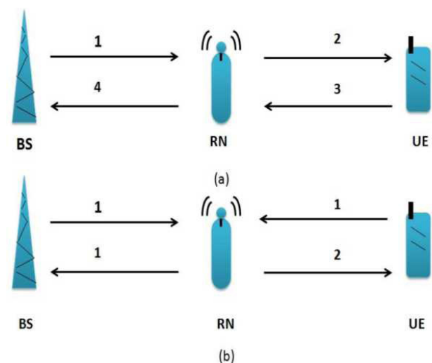
Figure 2. Relay transmission schemes. (a) Traditional 4TS scheme. (b) PNC scheme.
