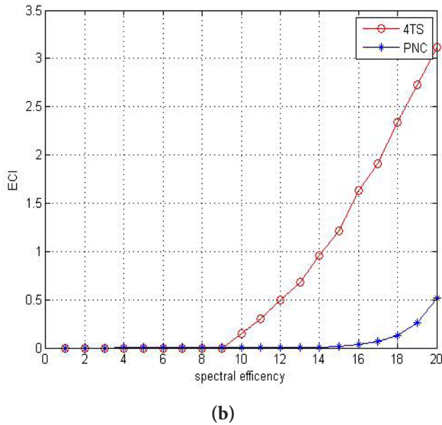
Figure 4. (a) Energy Consumption Index versus Spectral Efficiency when a = 4.5 and \beta = 0.3 . (b) Energy Consumption Index versus Spectral Efficiency when a = 4.5 and \beta = 0.8 .
