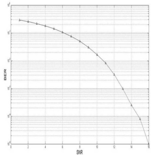
Figure 3. BER Vs. SNR graph of PNC with Slepian-Wolf compression.
