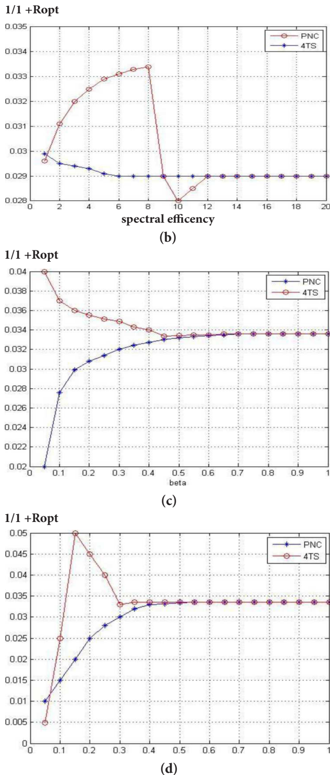
Figure 6. (a) Optimal Relay Development versus Spectral Efficiency when \beta = 0.4 . (b) Optimal Relay Development versus Spectral Efficiency when \beta = 0.7 . (c) \beta versus Optimal Relay Development when Spectral Efficiency is 3bps/Hz. (d) \beta versus Optimal Relay Development when Spectral Efficiency is 8bps/Hz.
