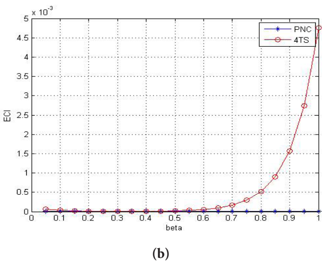
Figure 5. (a) Energy Comparison Index versus \beta when a = 4.5 and Spectral Efficiency is 2bps/Hz. (b) Energy Comparison Index versus \beta when a = 4.5 and Spectral Efficiency is 8bps/Hz.
