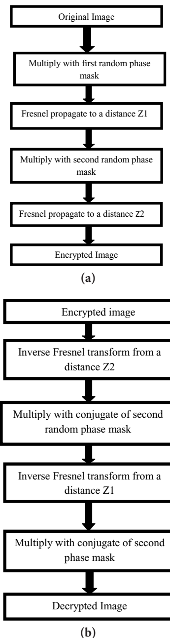
Figure 2. (a) Encoding process of double random phase Fresnel plane encoding and (b) Decoding process of double random phase Fresnel plane encoding.
