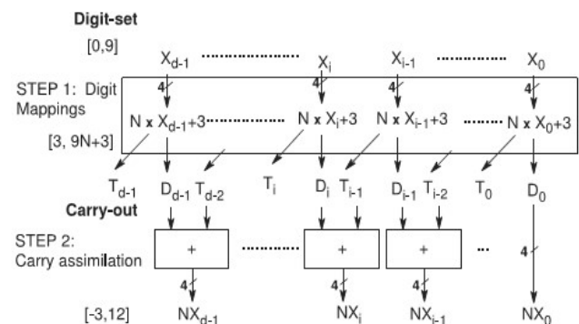
Figure 3. Decimal multiples NX generation.
