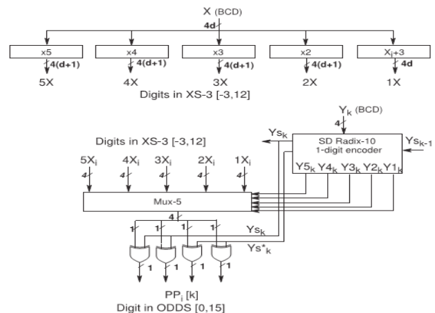
Figure 2. Generation of SD radix-10 partial product.
