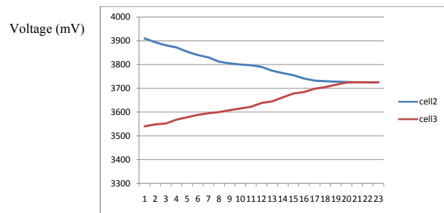
Figure 11. Cell balancing between cell 2 and cell3.
