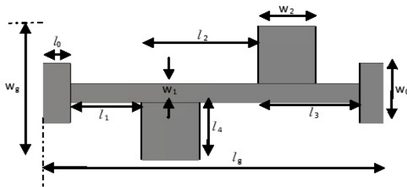
Figure 2. Geometry of elliptic function micro strip low pass structure.
