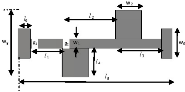
Figure 4. Geometry of UWB micro strip band pass filter, Simulated structure.
