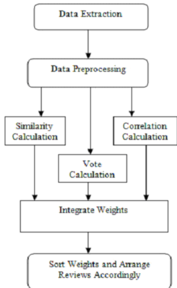
Figure 1. Flow diagram for calculating review relevance.
