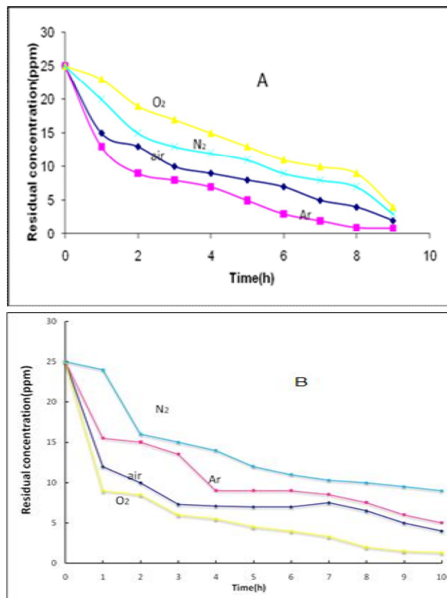
Fig. 2. Residual concentration of Direct Yellow 86 dye (25ppm), in de-ionized water after photocatalytic decolorization under UV irradiation in alkaline medium(pH=10)(A) and neutral pH(B) under various atmosphere.
