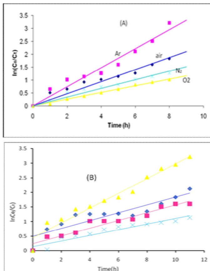
Fig.3. \ln(C_0/C_t) versus time(h) for photocatalytic decolorization under UV irradiation in alkaline medium(pH=10)(A) and neutral pH(B) under various atmosphere.
