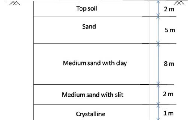
Fig. 4. Lithology of Besant nagar.
